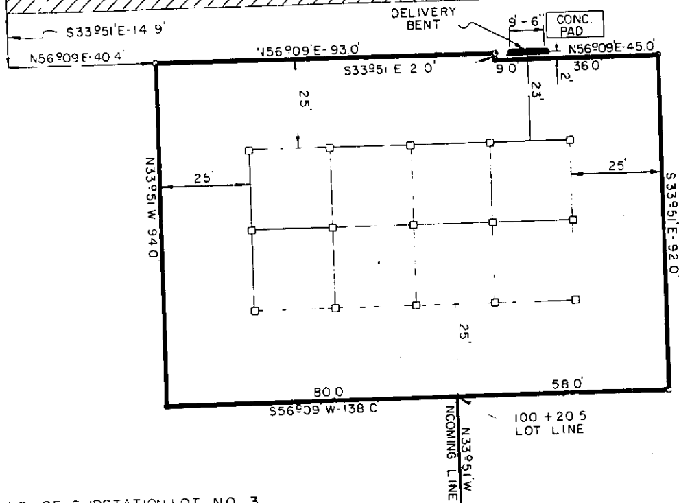
DETAILS OF SUBSTATION LOT NO. 3 SCALE: 1" = 30'
