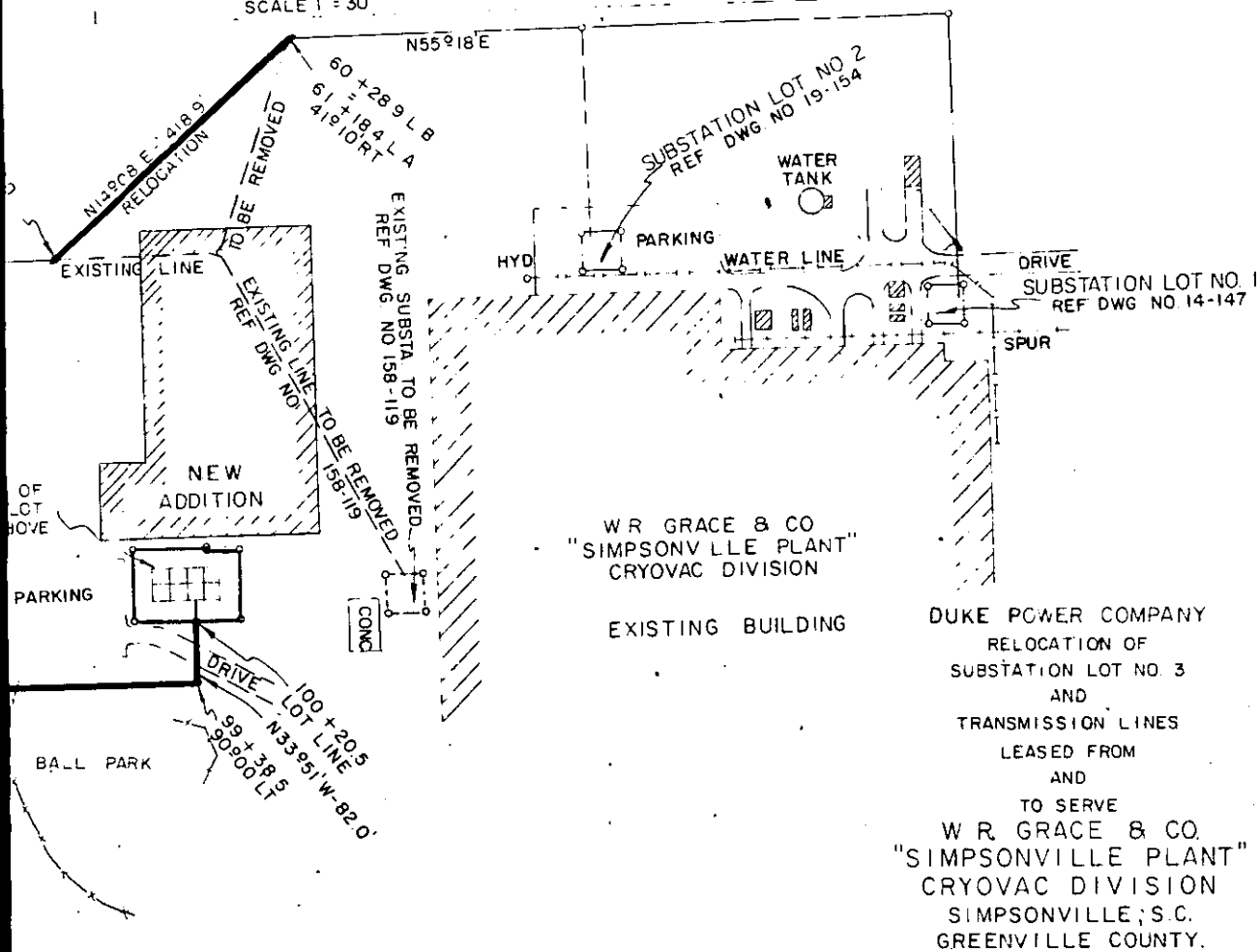
DETAILS OF SUBSTATION LOT NO. 3 SCALE: 1" = 30'
